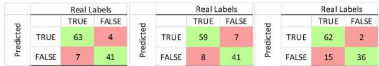
Figure 2. The performance results for the three lightweight CNN models.
