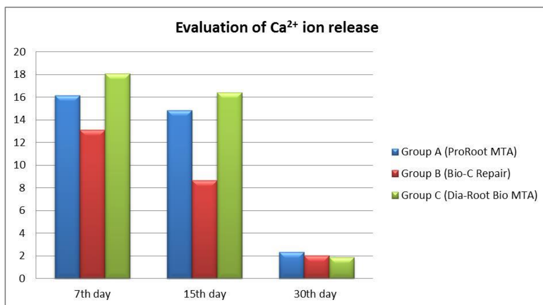
Figure 3. A graphical representation of mean \text{Ca}^{2+} release trend across the study groups over the experiment
