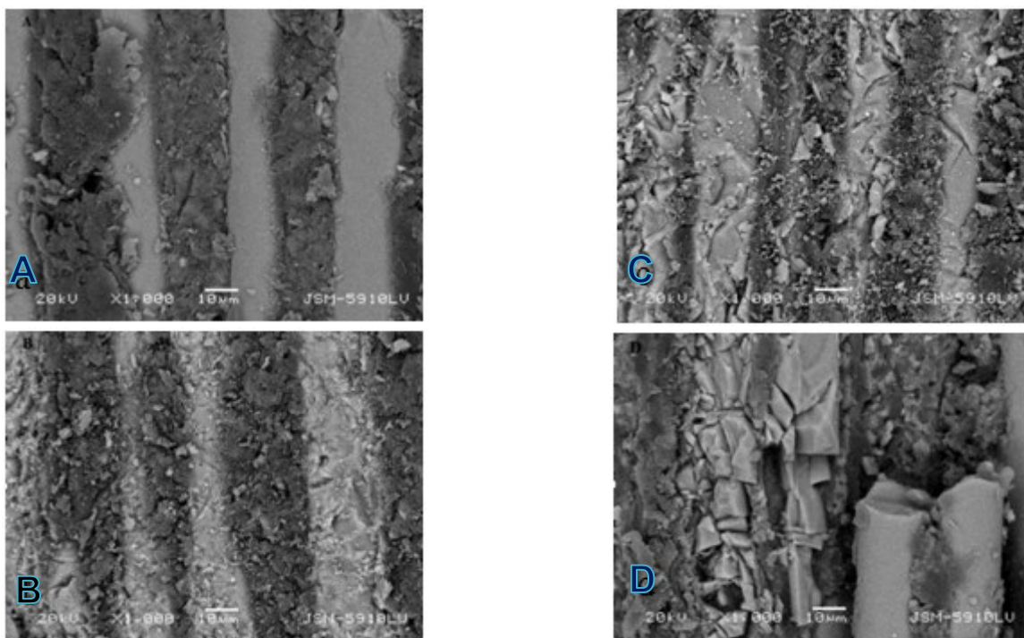
Figure 1. SEM images of post surfaces after surface treatment at X1000 magnification A= Control group, B= CoJet Sandblasting, C= Al 2 O 3 Sandblasting, and D=YbPL Laser
