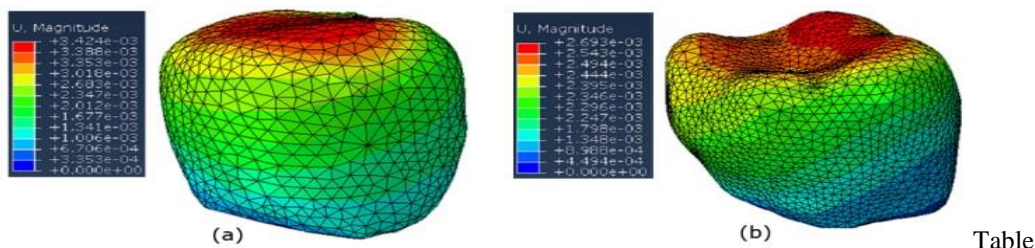
Figure 4. (a) Deformation distribution in normal first molar. (b) Deformation distribution in normal second molar.
