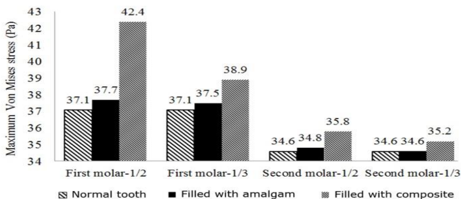
Figure 5. Comparison of maximum stress exerted on the first and second molars filled with amalgam and composite with filling depths equaling to 1/2 and 1/3 of the height of the normal tooth.
