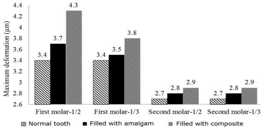
Figure 6. Comparison of maximum deformations exerted on the first and second molars filled with amalgam and composite with filling depths equaling to 1/2 and 1/3 of the height of the normal tooth.
